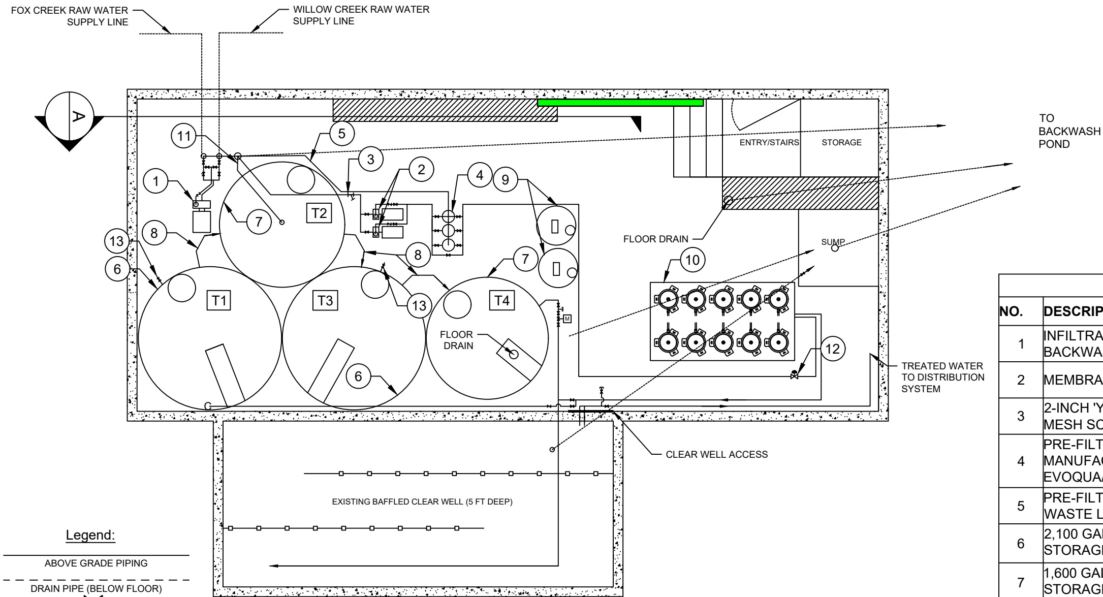
A PLAN VIEW SCALE: 1" = 5'
